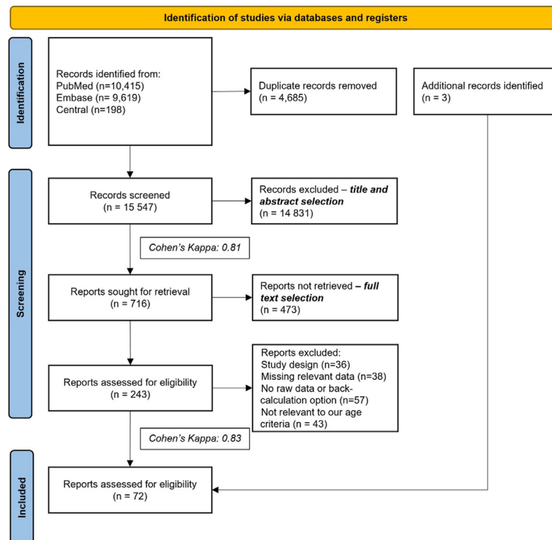
FIGURE 1 PRISMA 2020 flowchart representing the study selection process
